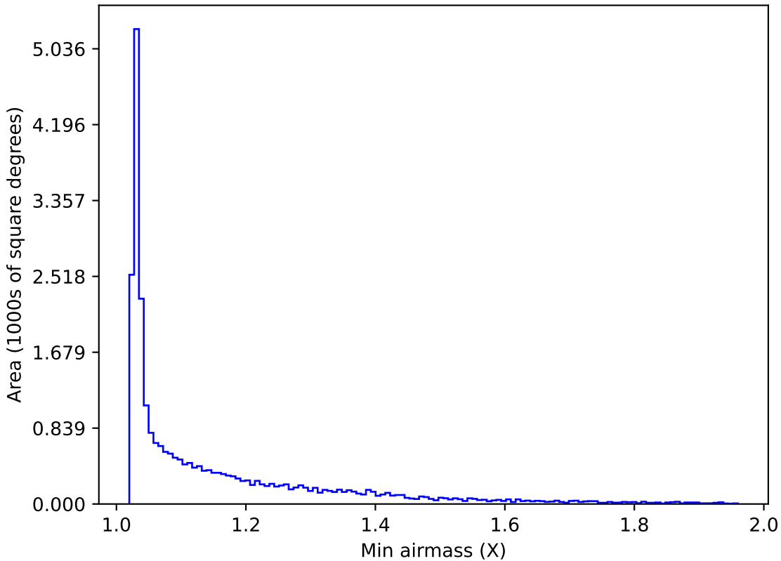
too_100_4v3.4_10yrs Yr 1 all bands: Min airmass
