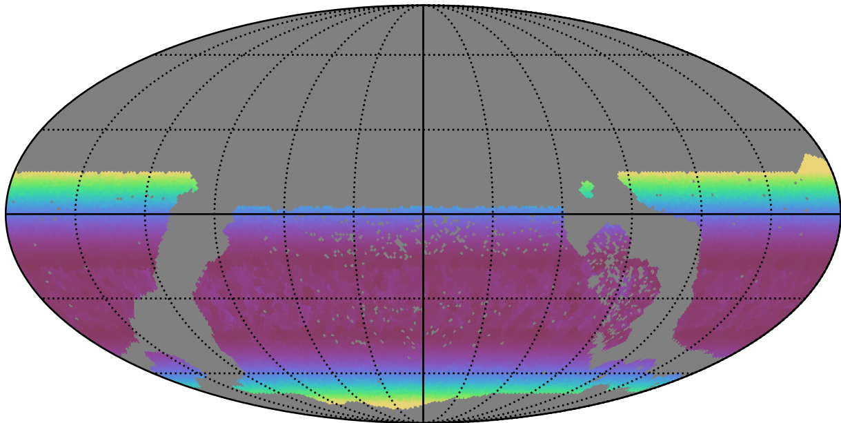
too_100_4v3.4_10yrs WFD u band: Min airmass
