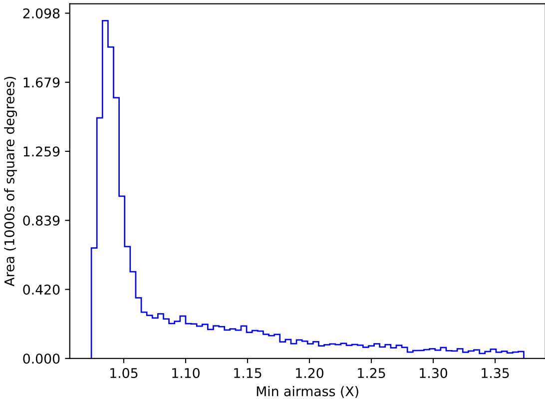
too_100_4v3.4_10yrs WFD u band: Min airmass
