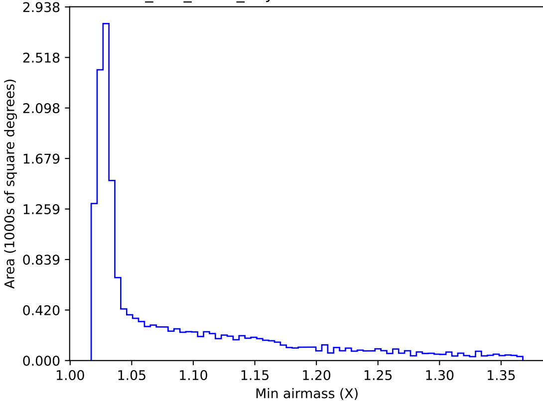
too_100_4v3.4_10yrs WFD r band: Min airmass
