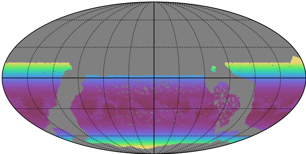
too_100_4v3.4_10yrs WFD g band: Min airmass
