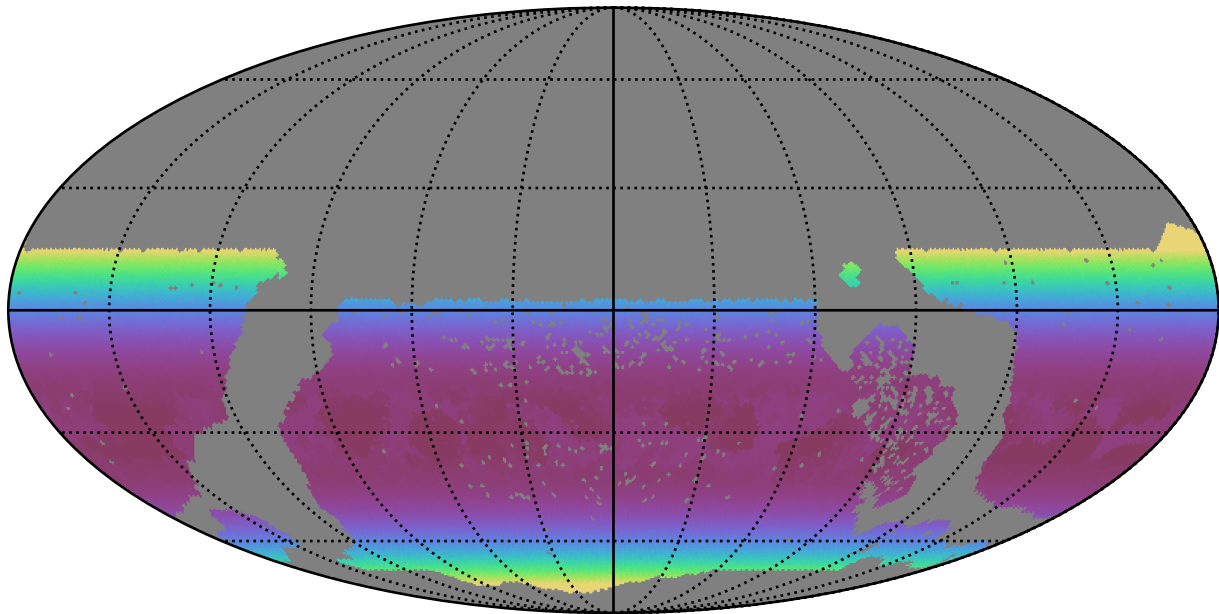
too_100_4v3.4_10yrs WFD all bands: Min airmass
