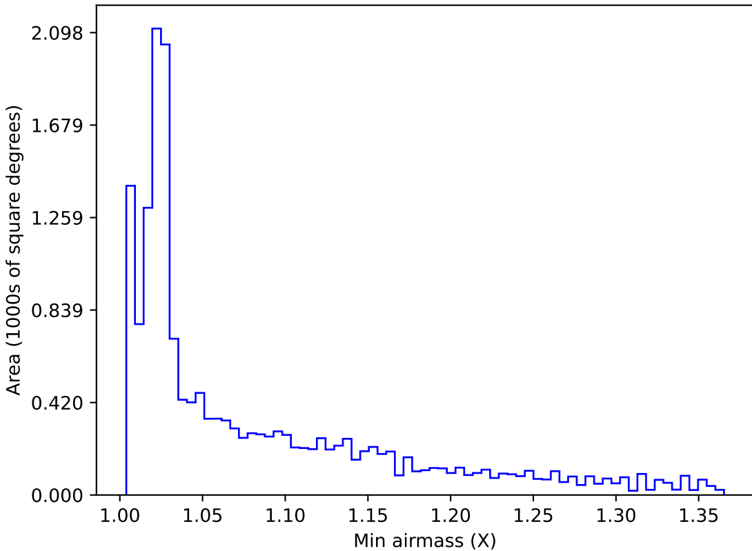
too_100_4v3.4_10yrs WFD all bands: Min airmass
