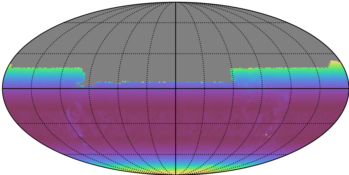
too_100_4v3.4_10yrs All sky u band: Min airmass
