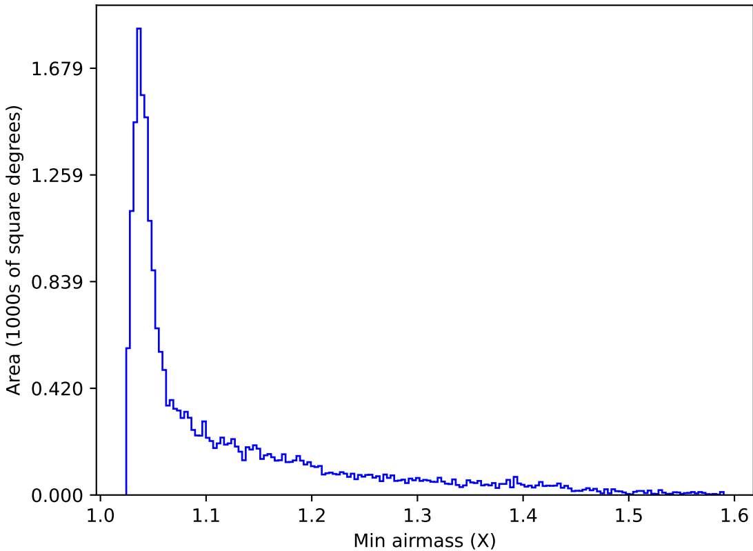
too_100_4v3.4_10yrs All sky u band: Min airmass
