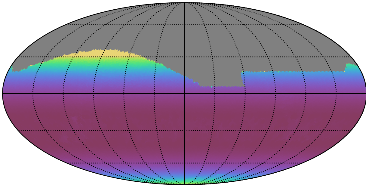
too_100_4v3.4_10yrs All sky r band: Min airmass
