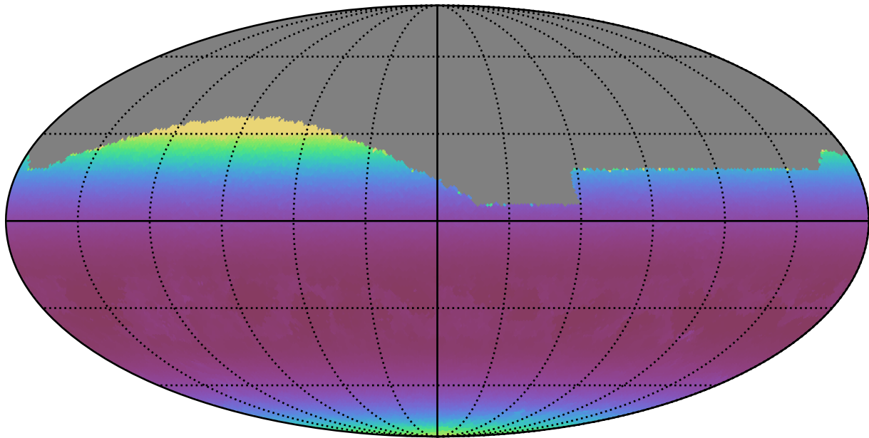
too_100_4v3.4_10yrs All sky g band: Min airmass
