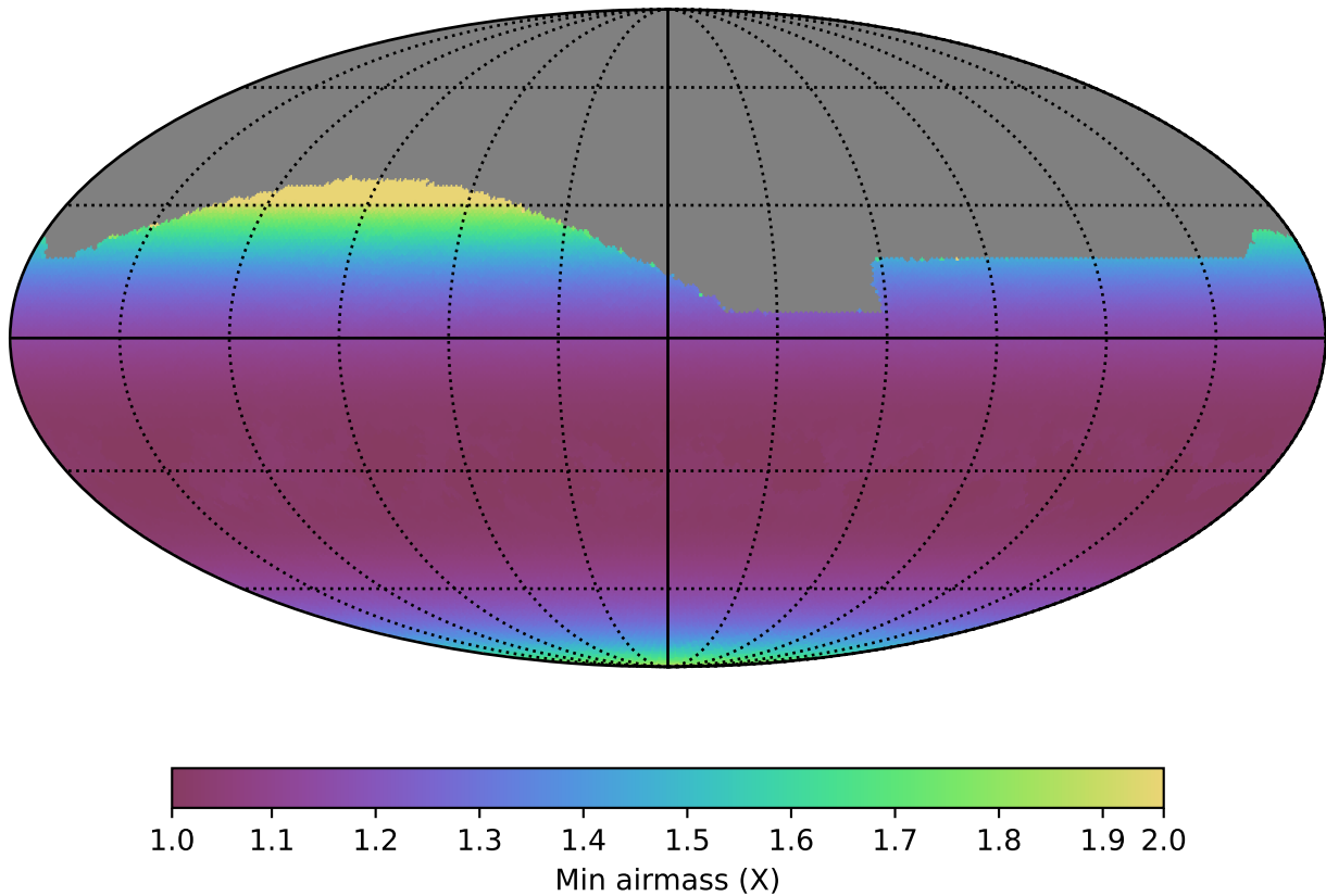
too_100_4v3.4_10yrs All sky all bands: Min airmass
