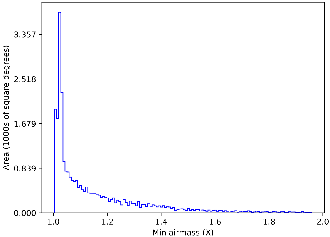
too_100_4v3.4_10yrs All sky all bands: Min airmass
