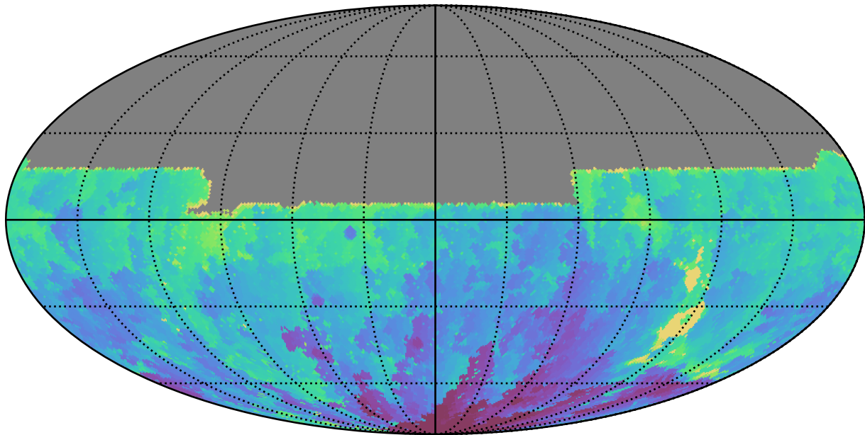
too_100_4v3.4_10yrs All sky u band: Min HA
