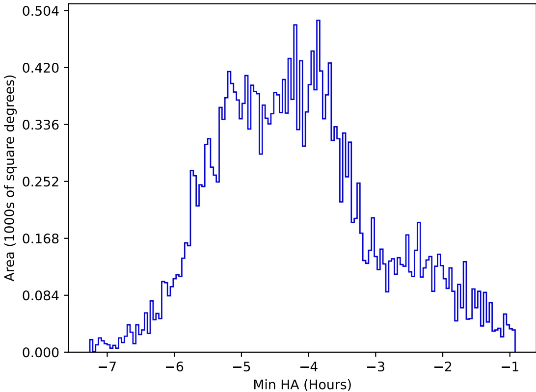
too_100_4v3.4_10yrs All sky r band: Min HA
