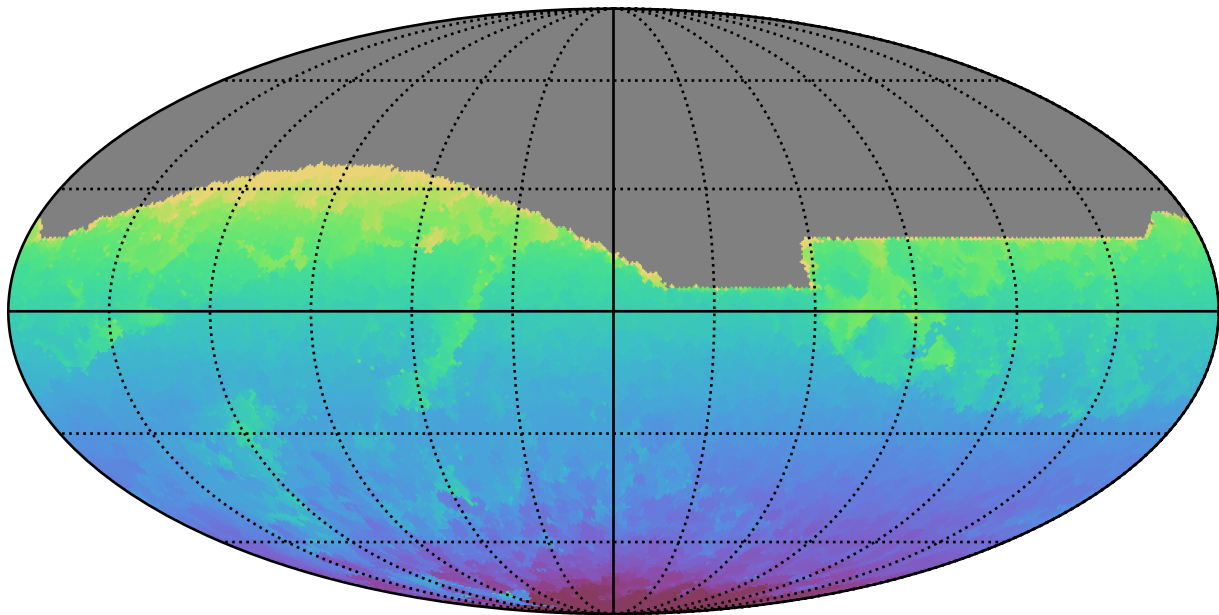
too_100_4v3.4_10yrs All sky all bands: Min HA
