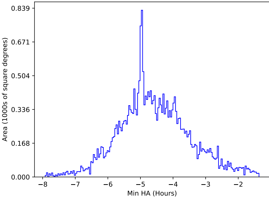
too_100_4v3.4_10yrs All sky all bands: Min HA
