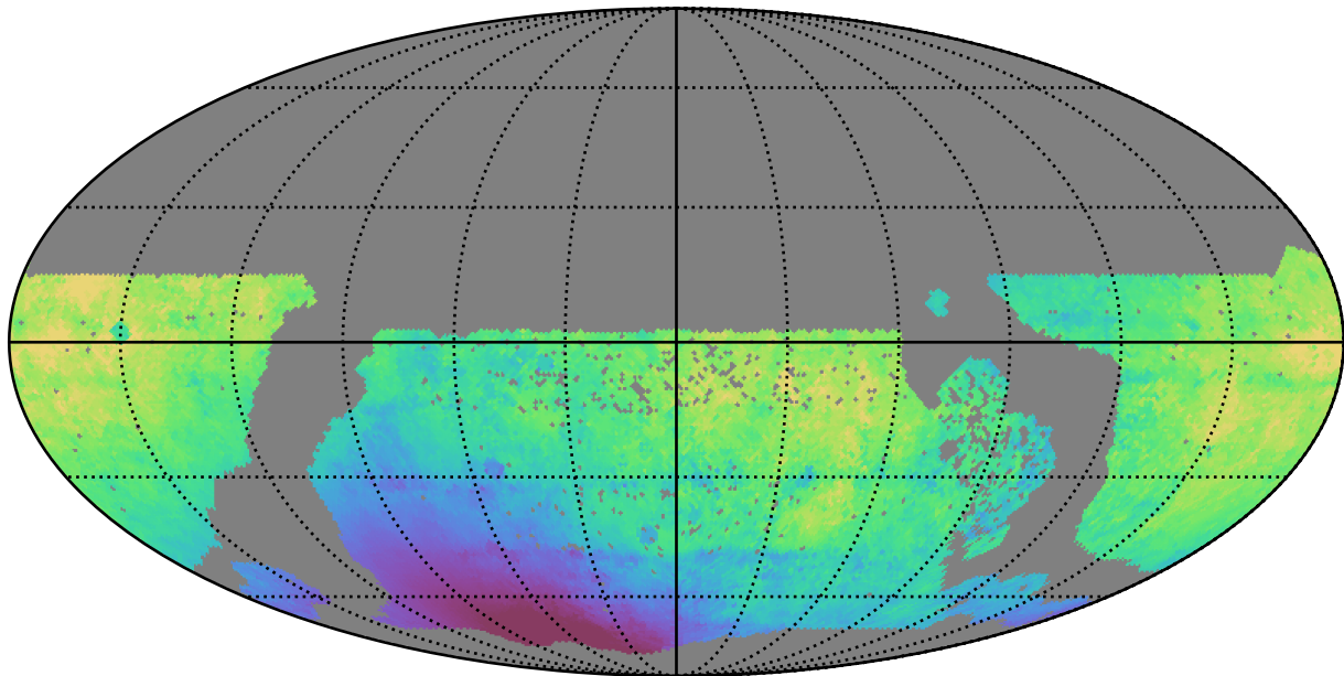
too_100_4v3.4_10yrs WFD z band: Median solarElong
