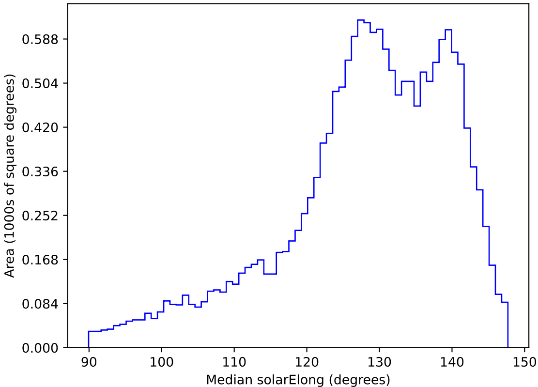
too_100_4v3.4_10yrs WFD z band: Median solarElong
