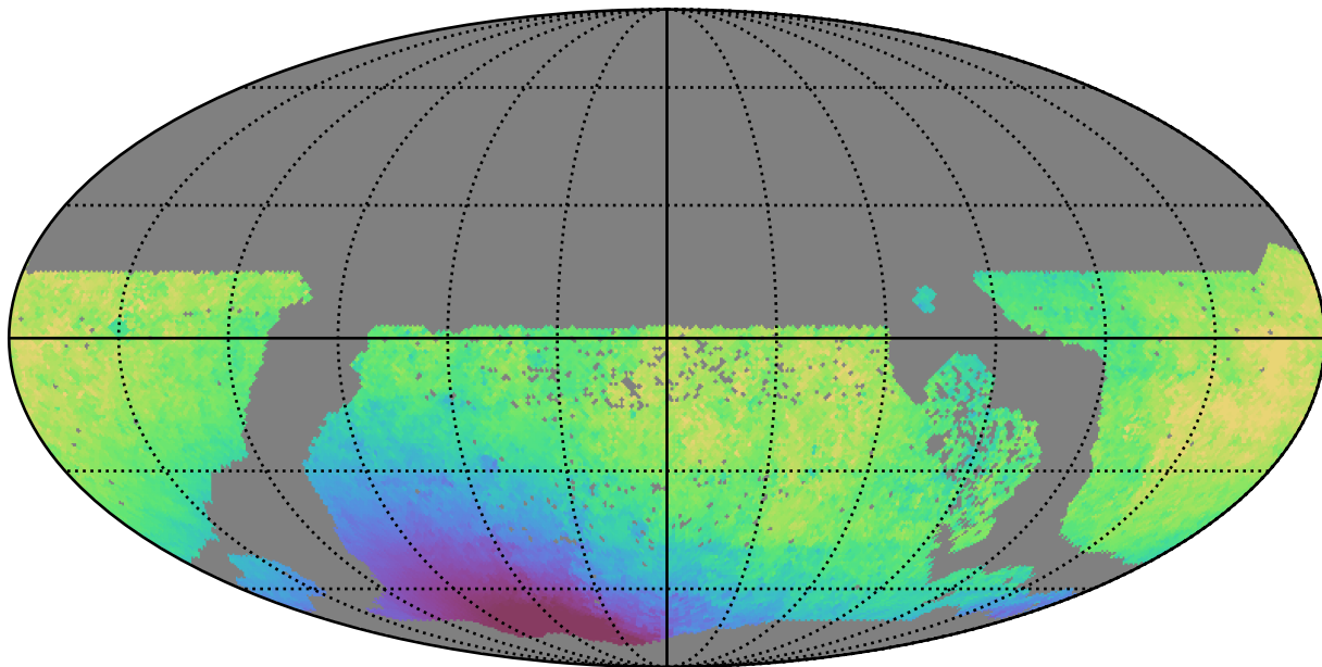
too_100_4v3.4_10yrs WFD y band: Median solarElong
