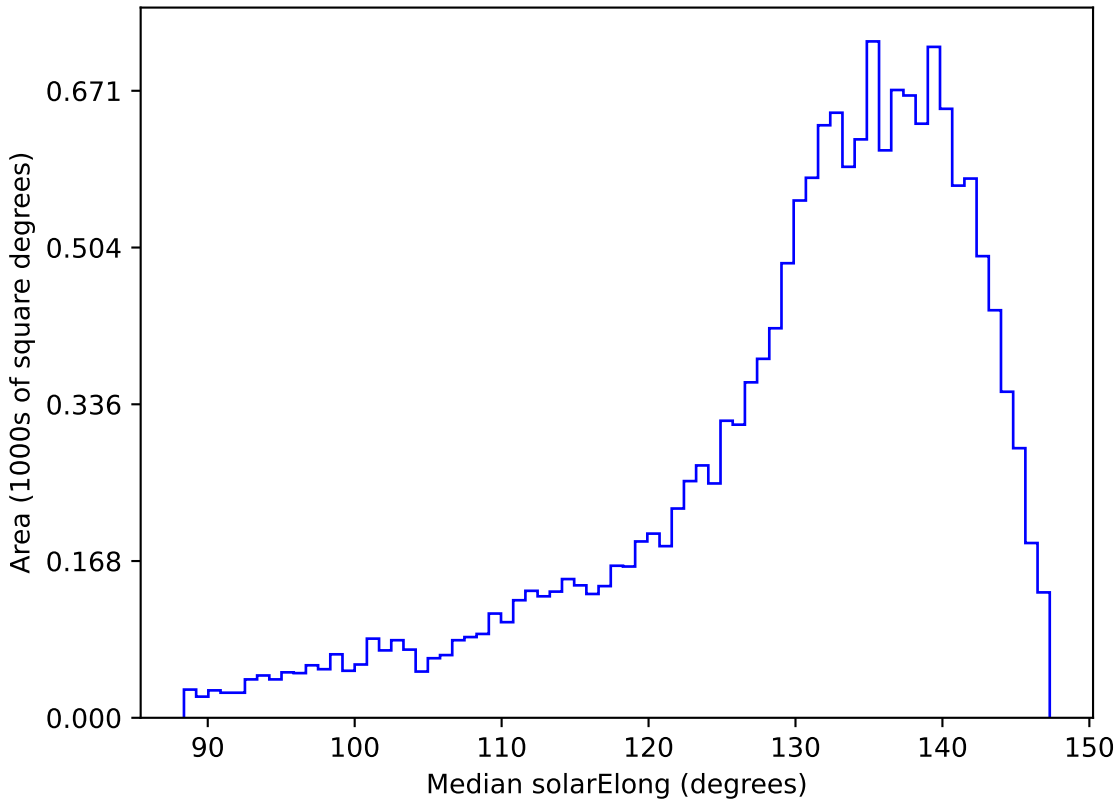
too_100_4v3.4_10yrs WFD y band: Median solarElong
