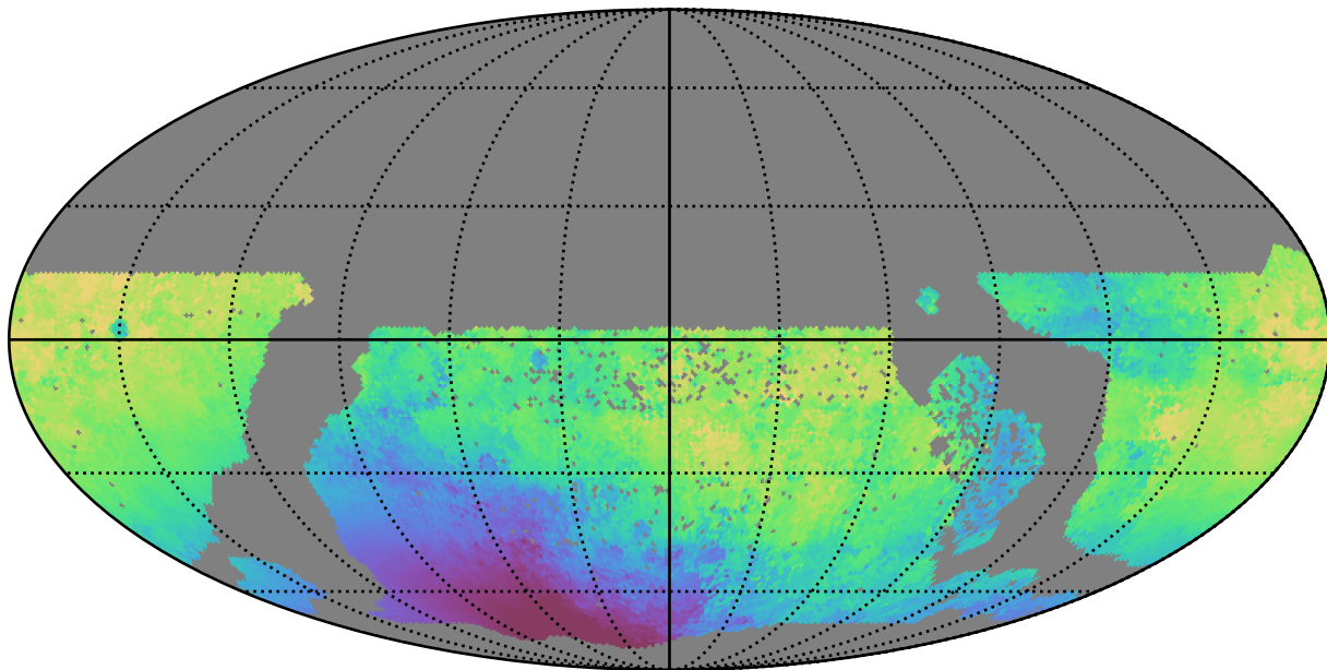
too_100_4v3.4_10yrs WFD u band: Median solarElong
