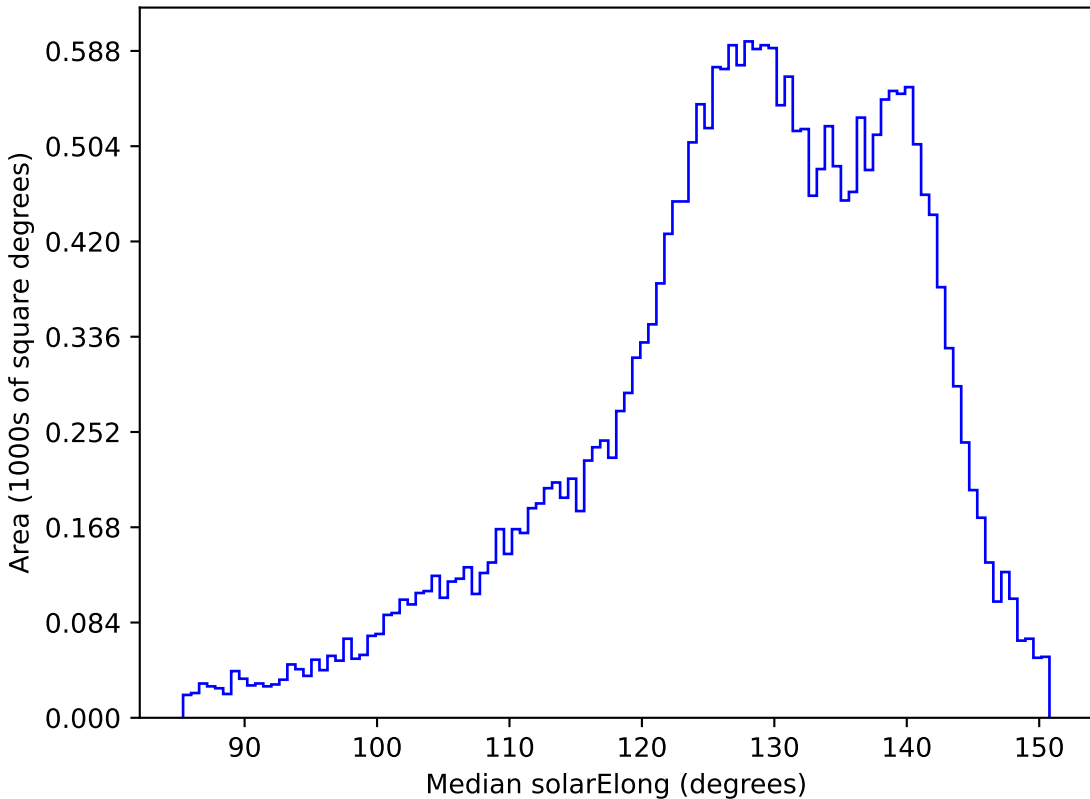
too_100_4v3.4_10yrs All sky z band: Median solarElong
