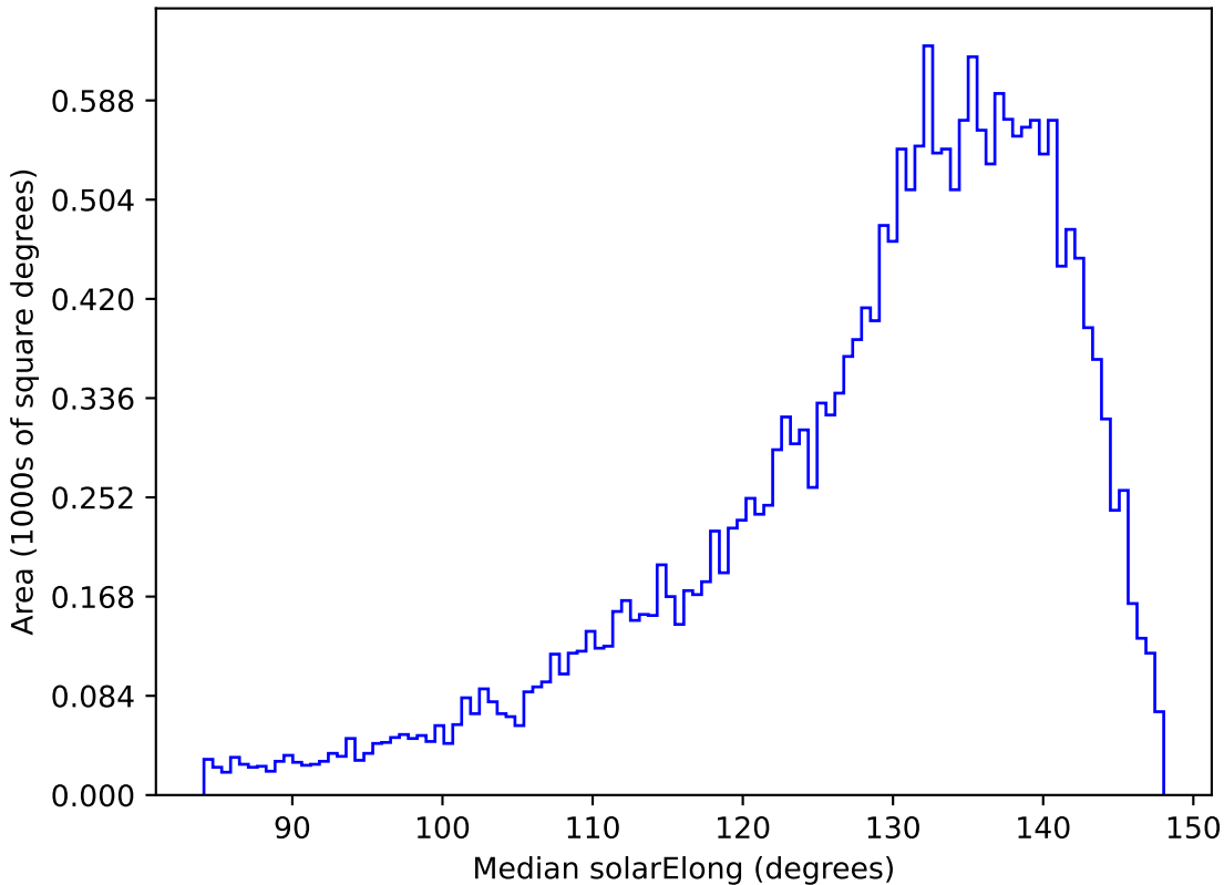
too_100_4v3.4_10yrs All sky y band: Median solarElong
