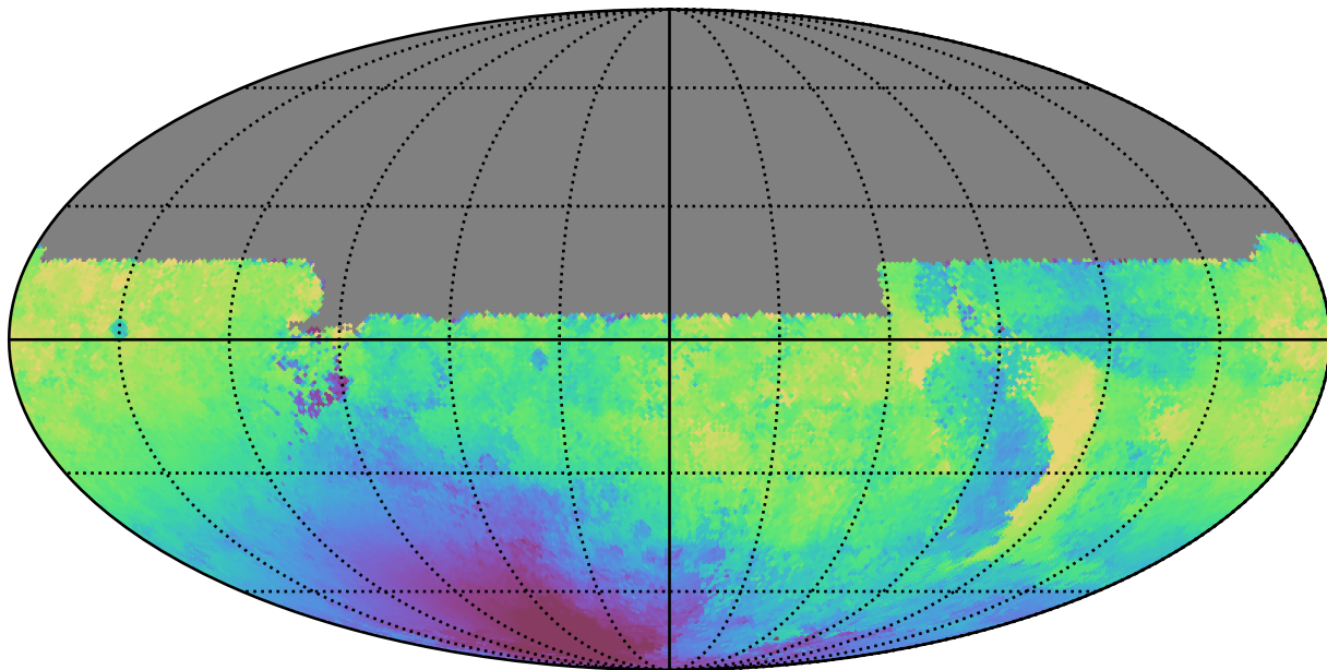
too_100_4v3.4_10yrs All sky u band: Median solarElong
