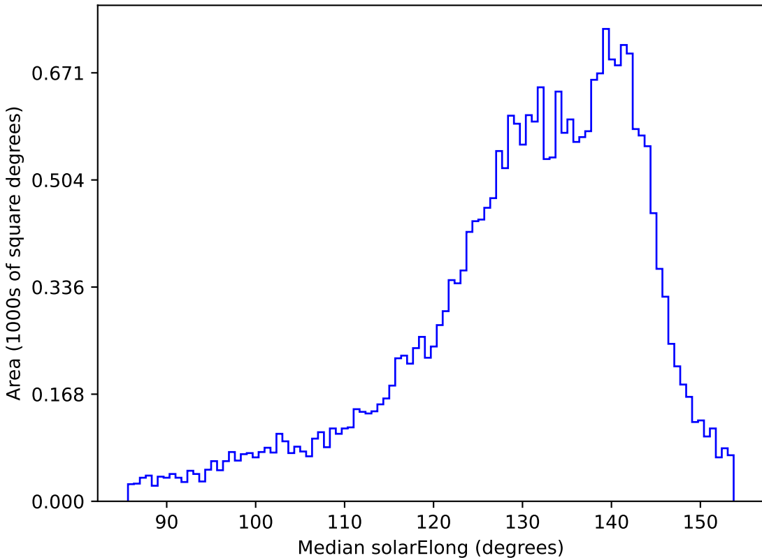
too_100_4v3.4_10yrs All sky r band: Median solarElong
