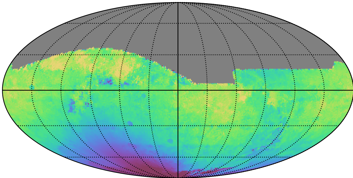
too_100_4v3.4_10yrs All sky i band: Median solarElong
