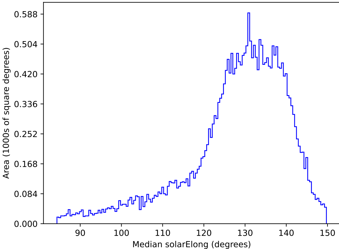
too_100_4v3.4_10yrs All sky i band: Median solarElong
