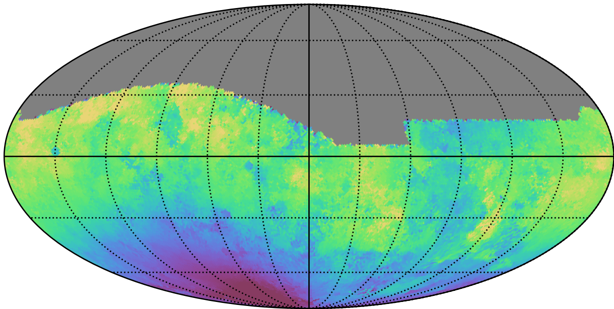
too_100_4v3.4_10yrs All sky g band: Median solarElong
