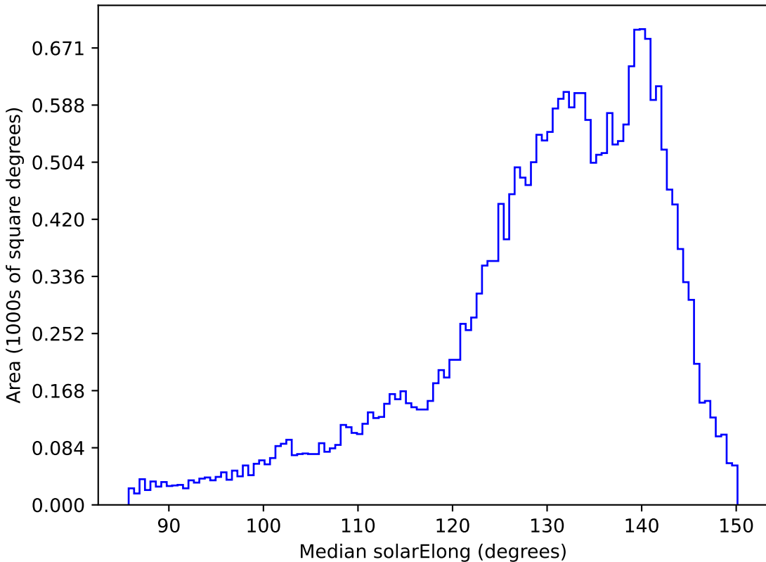
too_100_4v3.4_10yrs All sky all bands: Median solarElong
