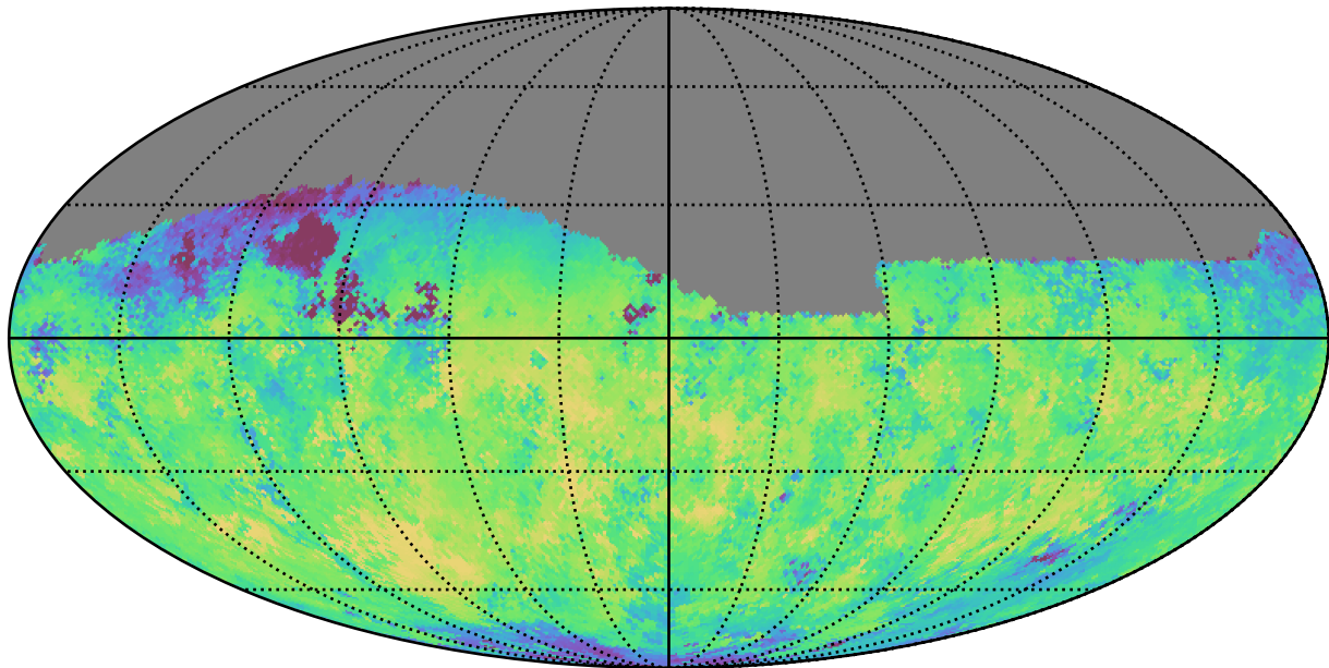
too_100_4v3.4_10yrs Yr 1 z band: Median skyBrightness
