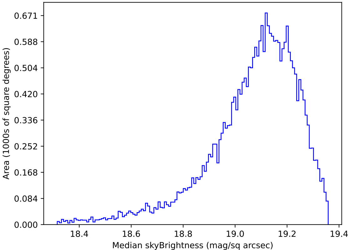
too_100_4v3.4_10yrs Yr 1 z band: Median skyBrightness
