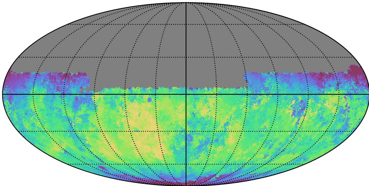
too_100_4v3.4_10yrs Yr 1 y band: Median skyBrightness
