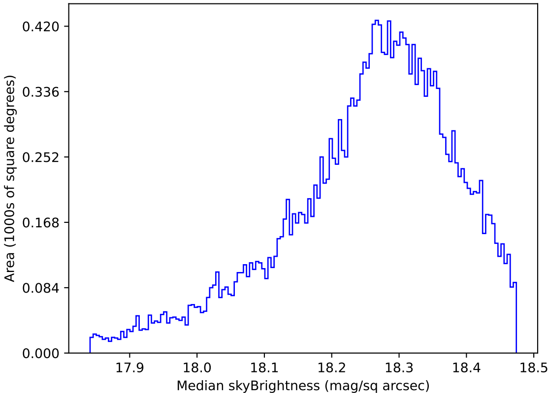
too_100_4v3.4_10yrs Yr 1 y band: Median skyBrightness
