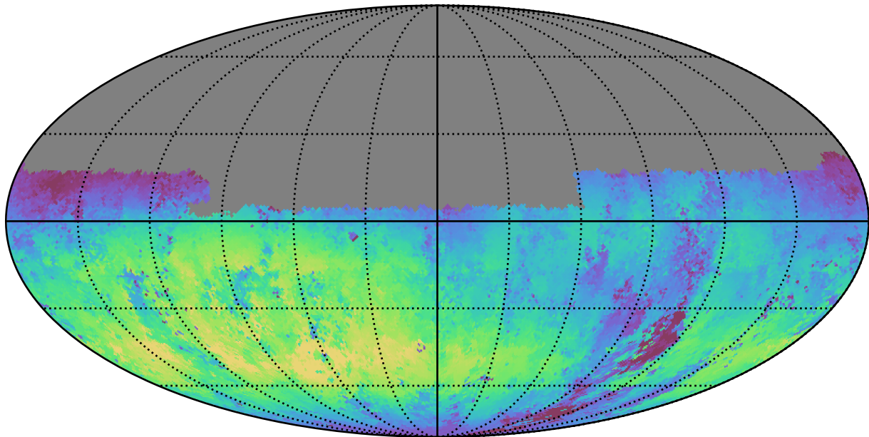
too_100_4v3.4_10yrs Yr 1 u band: Median skyBrightness
