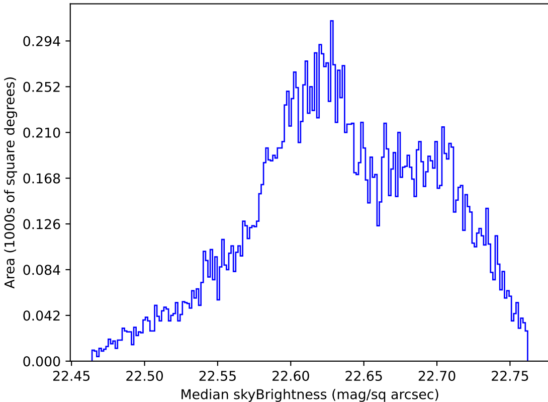
too_100_4v3.4_10yrs Yr 1 u band: Median skyBrightness
