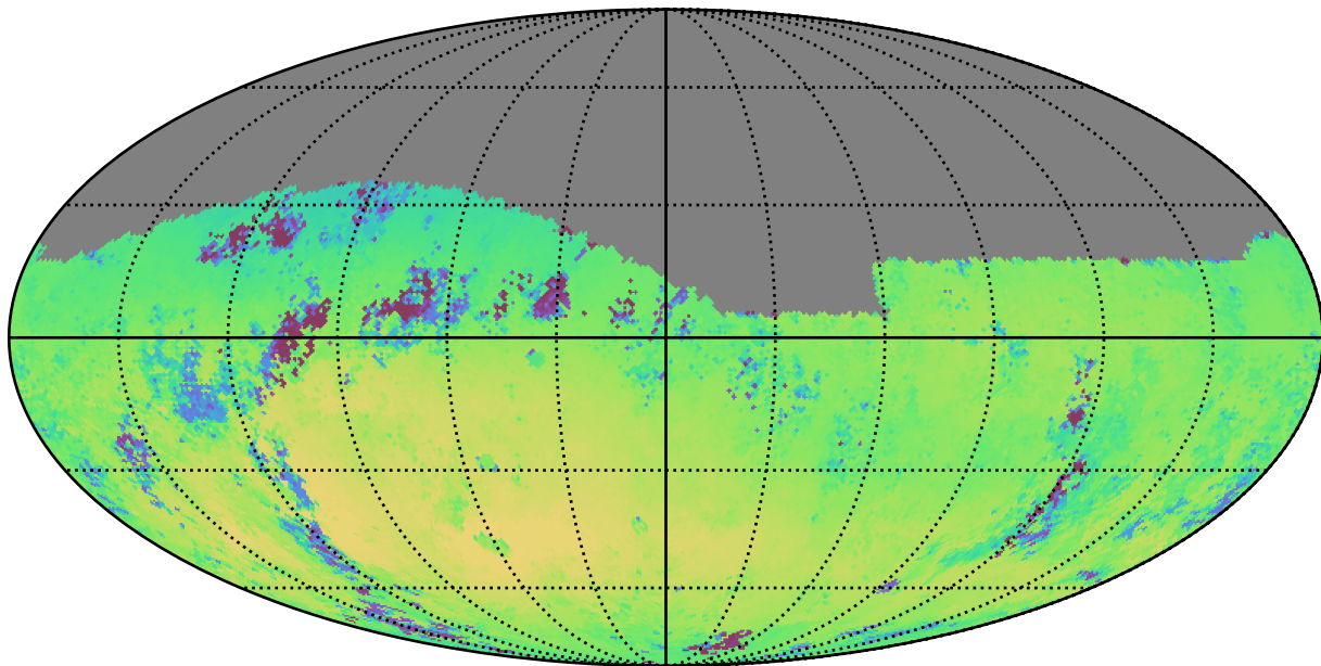
too_100_4v3.4_10yrs Yr 1 r band: Median skyBrightness
