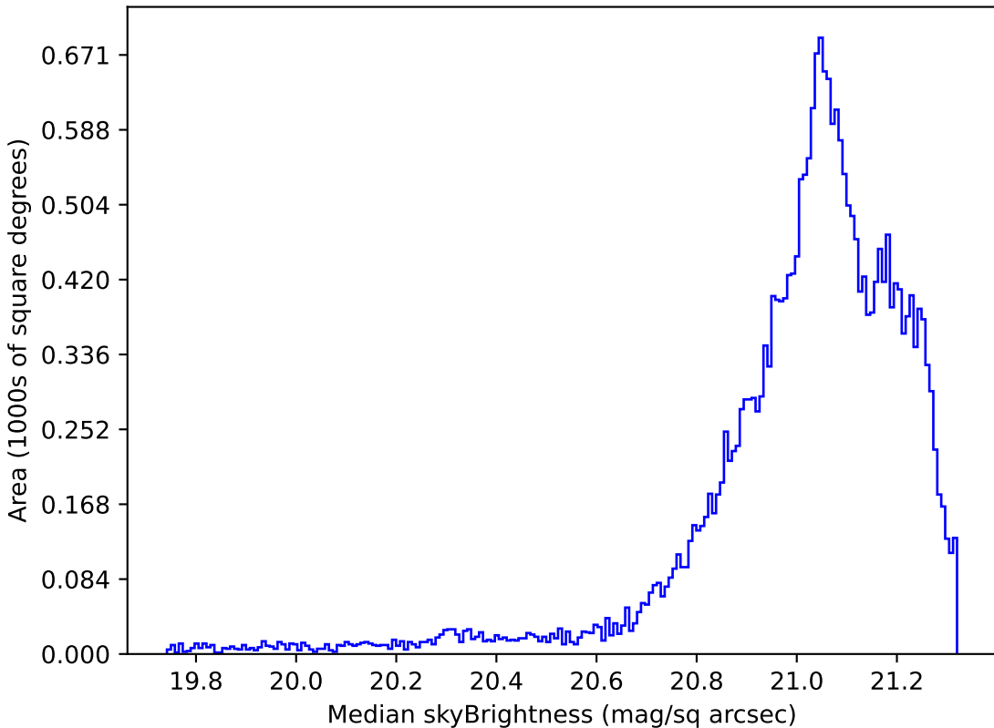
too_100_4v3.4_10yrs Yr 1 r band: Median skyBrightness
