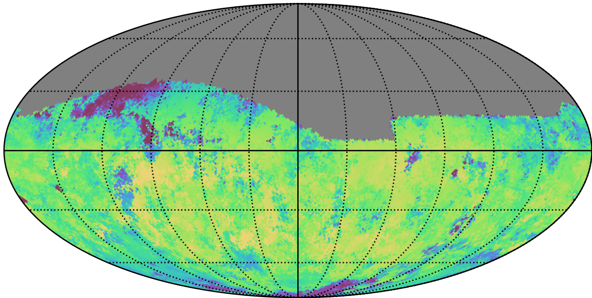
too_100_4v3.4_10yrs Yr 1 i band: Median skyBrightness
