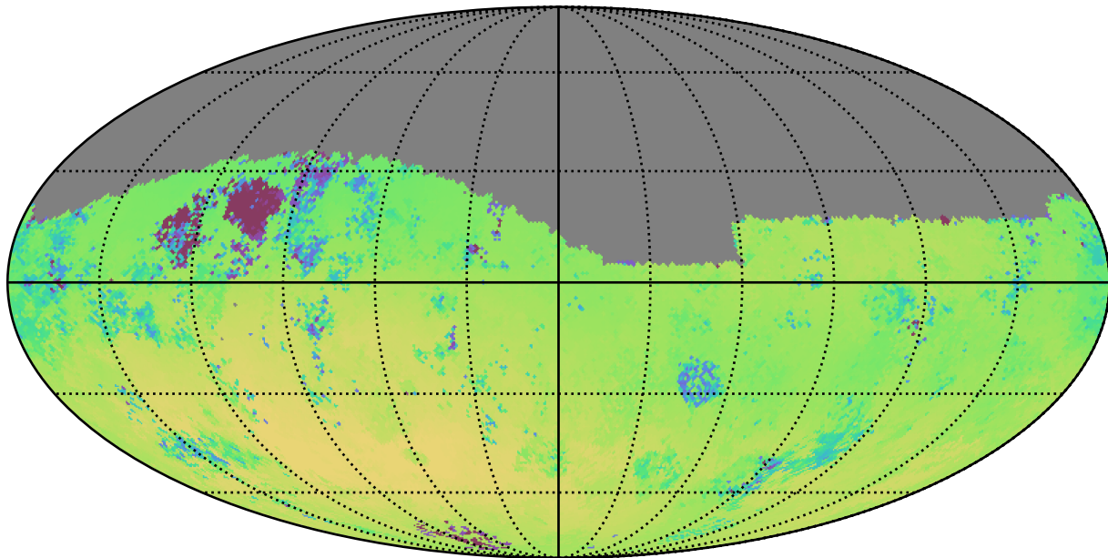
too_100_4v3.4_10yrs Yr 1 g band: Median skyBrightness
