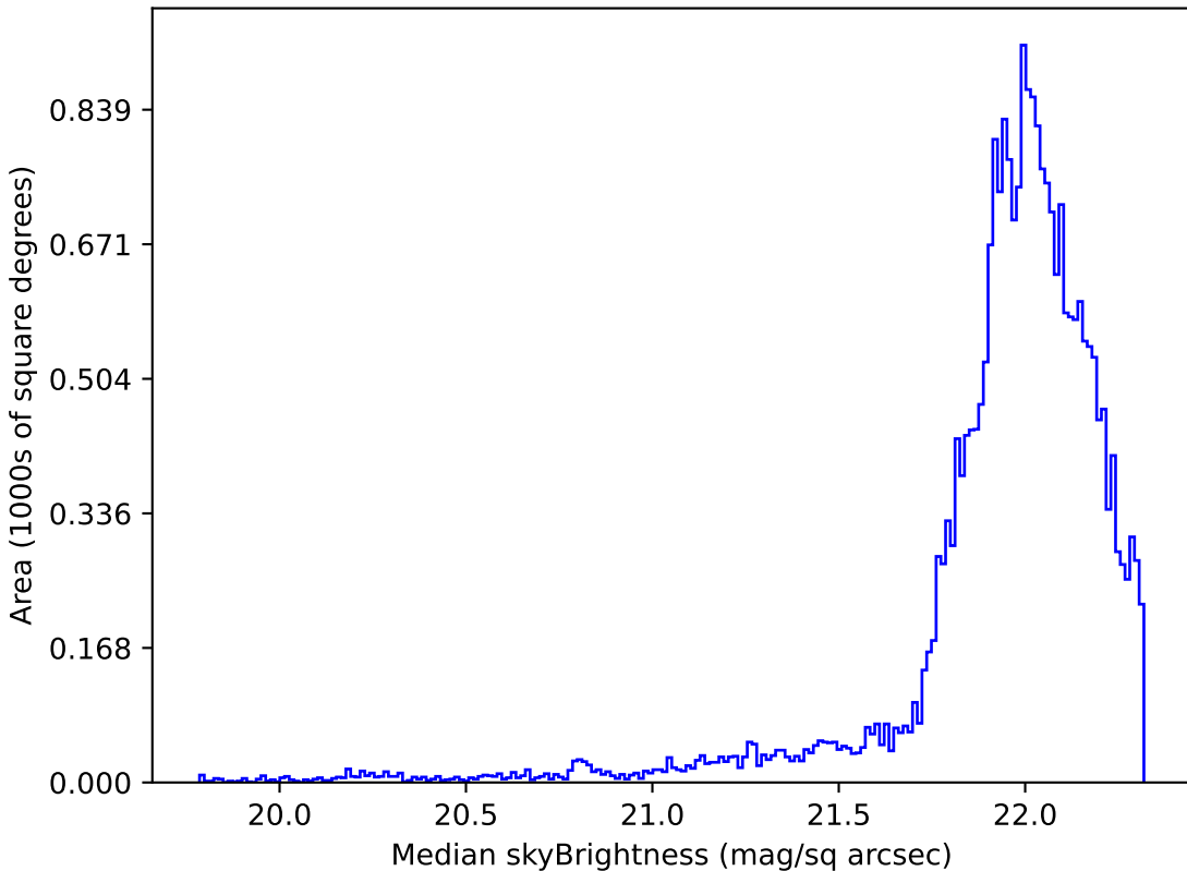
too_100_4v3.4_10yrs Yr 1 g band: Median skyBrightness
