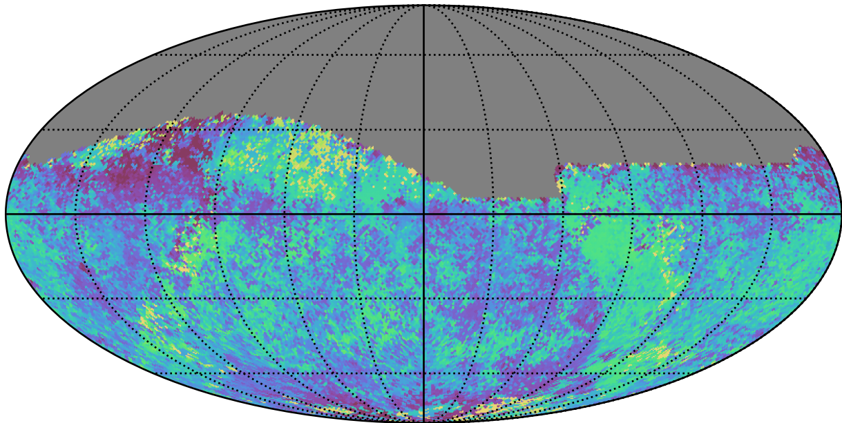
too_100_4v3.4_10yrs Yr 1 all bands: Median skyBrightness
