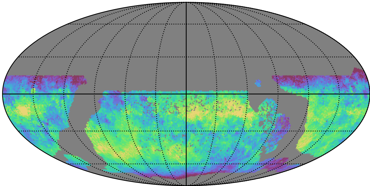
too_100_4v3.4_10yrs WFD z band: Median skyBrightness
