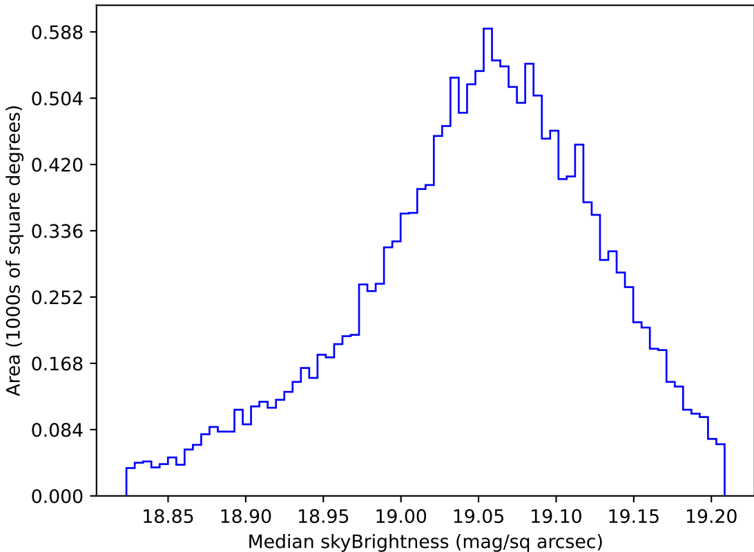
too_100_4v3.4_10yrs WFD z band: Median skyBrightness
