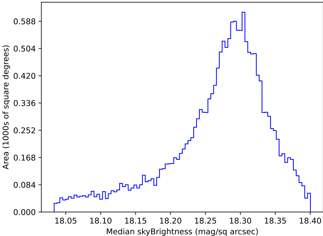
too_100_4v3.4_10yrs WFD y band: Median skyBrightness
