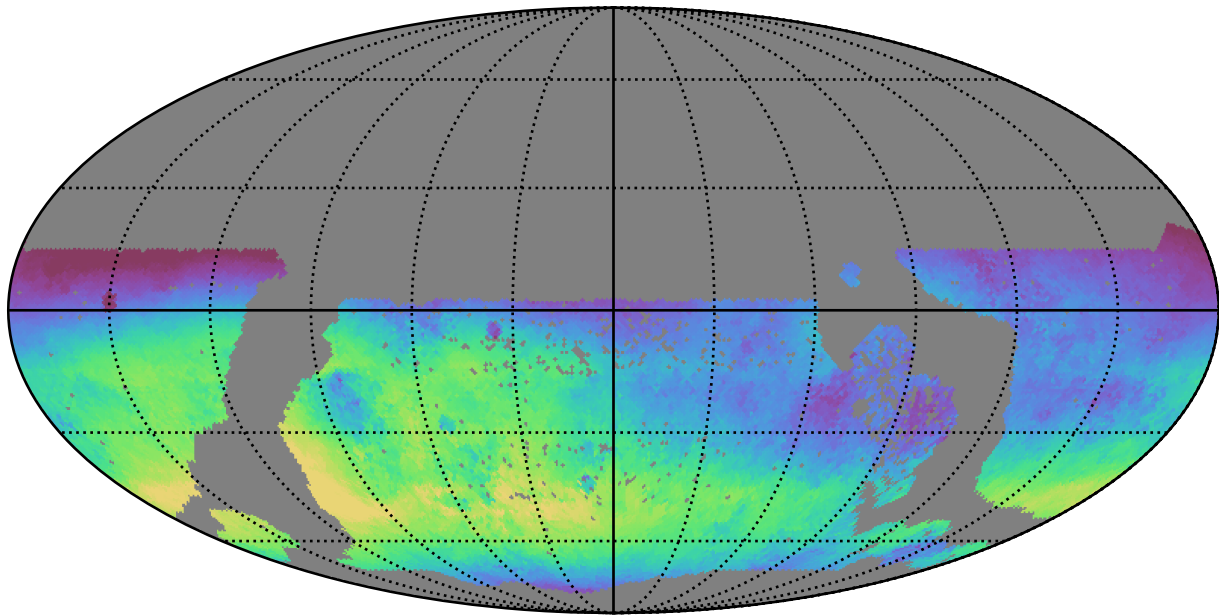
too_100_4v3.4_10yrs WFD u band: Median skyBrightness
