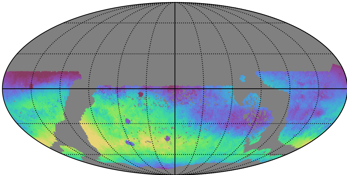
too_100_4v3.4_10yrs WFD r band: Median skyBrightness
