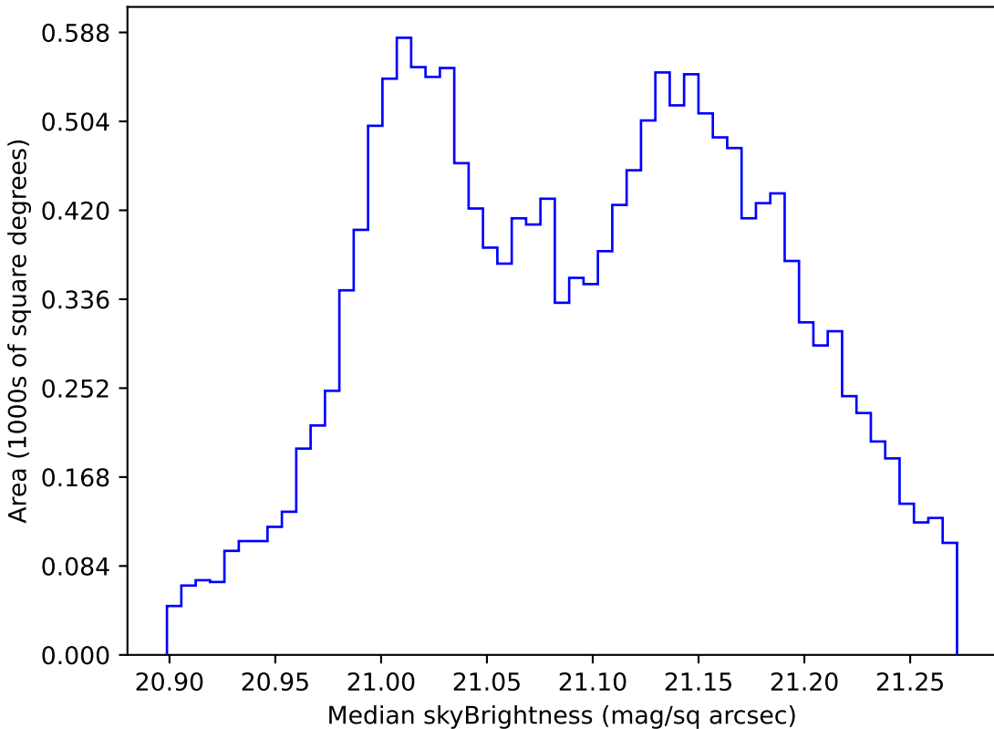
too_100_4v3.4_10yrs WFD r band: Median skyBrightness
