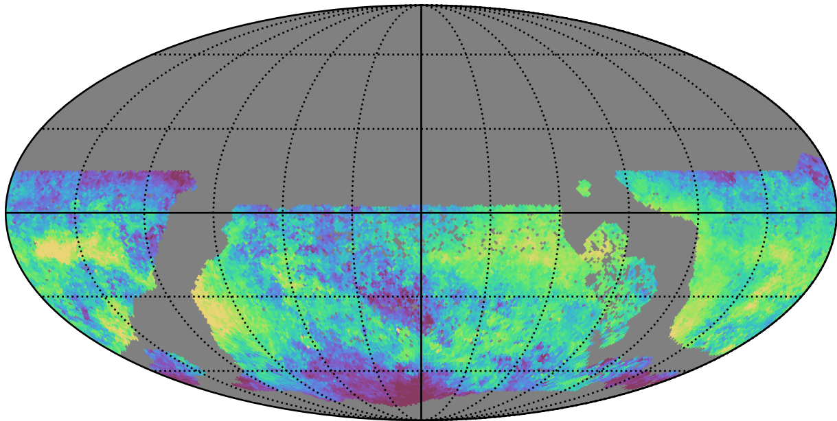
too_100_4v3.4_10yrs WFD i band: Median skyBrightness
