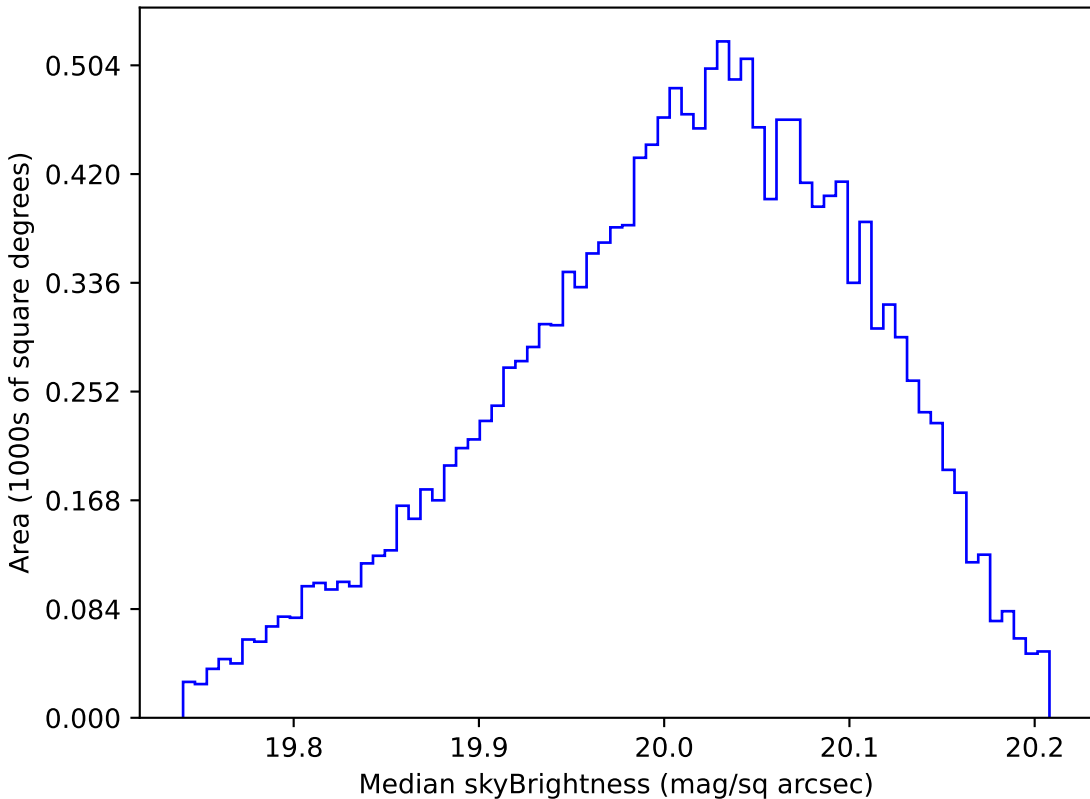
too_100_4v3.4_10yrs WFD i band: Median skyBrightness
